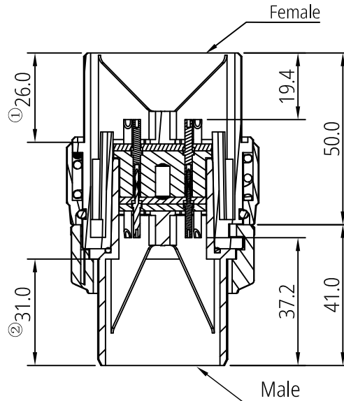
Mating View
