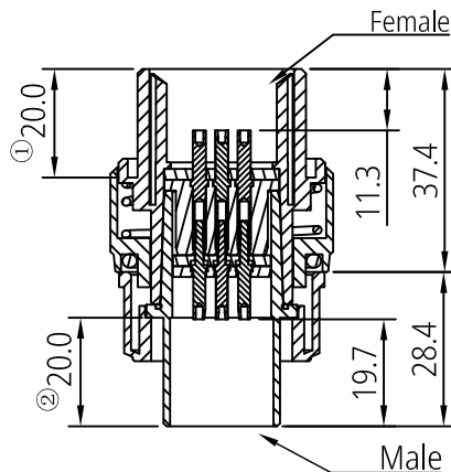
Mating View
