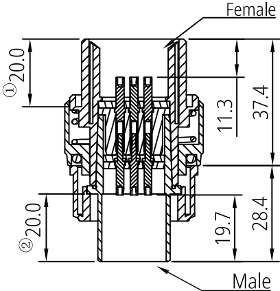
Mating View
