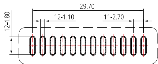
Recommended P.C.B layout (Top View) Tolerance ±0.05
